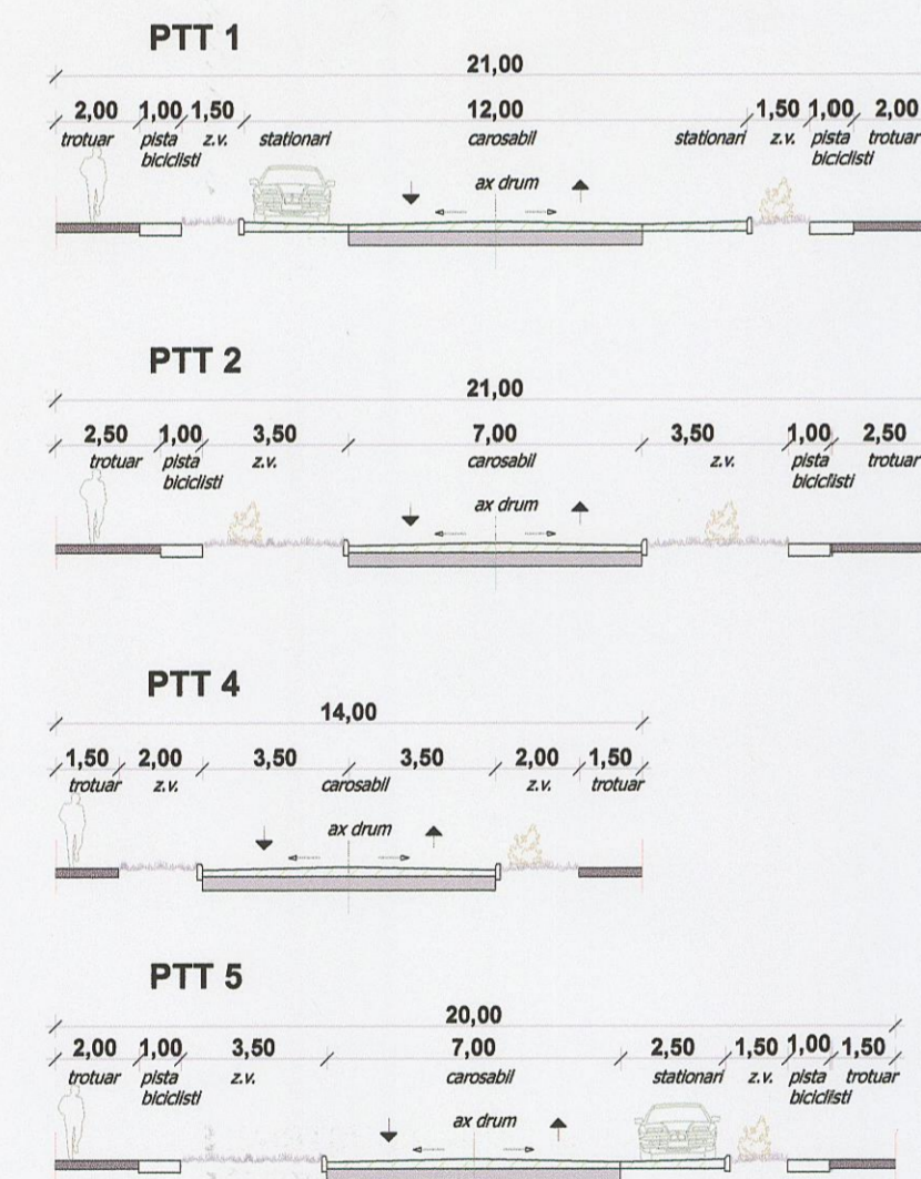
PROFILE CARACTERISTICE ( Sc 1/200 )
